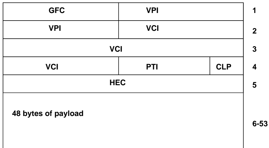
Figure 4-1 ATM Cell Format
