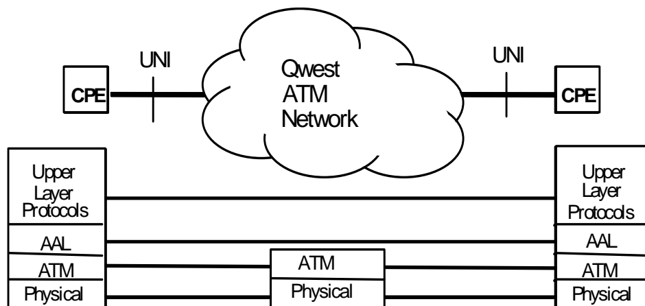
Figure 2-1 Qwest ATM Service Protocol Relationships
